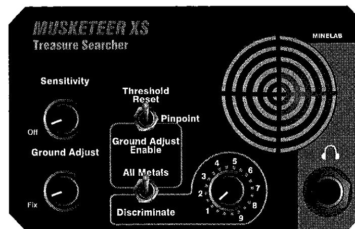
Figure 10 - The Minelab Musketeer XS and XS Pro Control Panel
