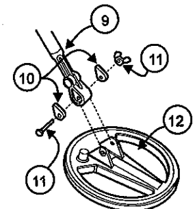
Figure 2 - The coil and lower shaft assembly
