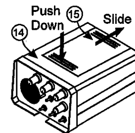
Figure 7 - Installing the NiCad Battery Pack
